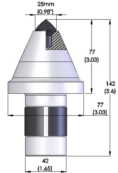
3. JZ77/42-WSM/M25-23-3
