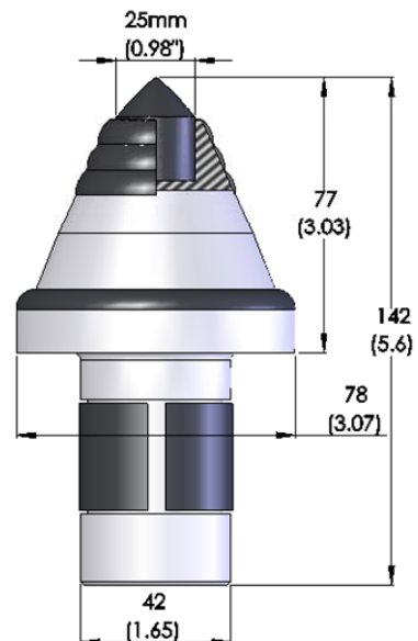
5. JZ77/42-WSM/Z25-42N-3
