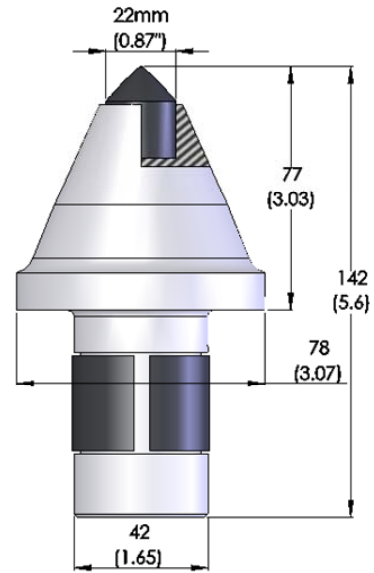
5. JZ77/42-WSM/Z25-42N-3
