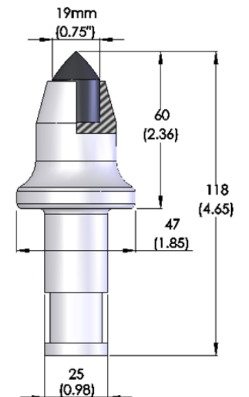
7. JZ60/25-C34FSR/Z19-42-3
