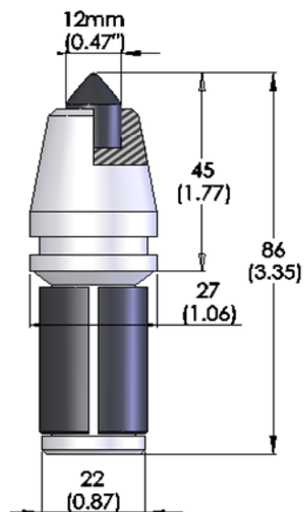
6. JZ43/19-K3LA/C16-42-3
