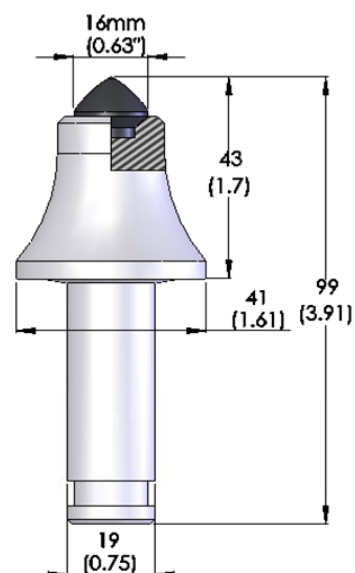
6. JZ43/19-K3LA/C16-42-3
