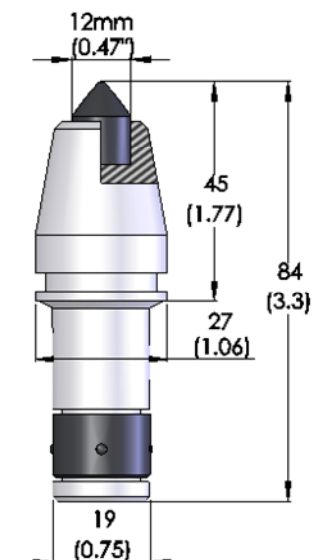
5. JZ45/19-C21HD/Z12-42-3
